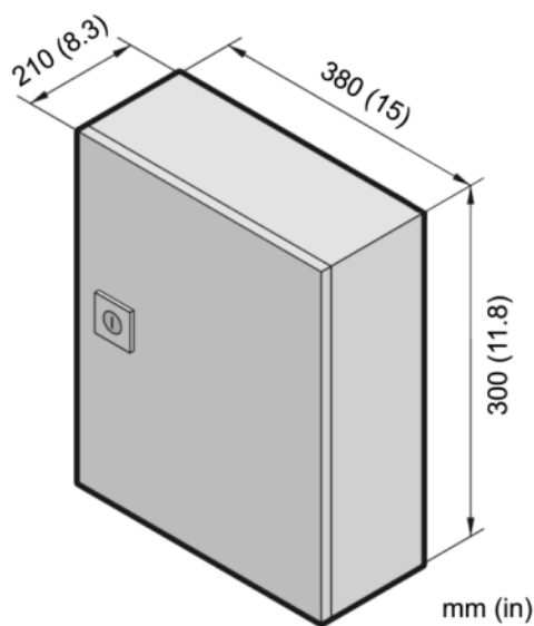
Figure 7-28: Junction Box
