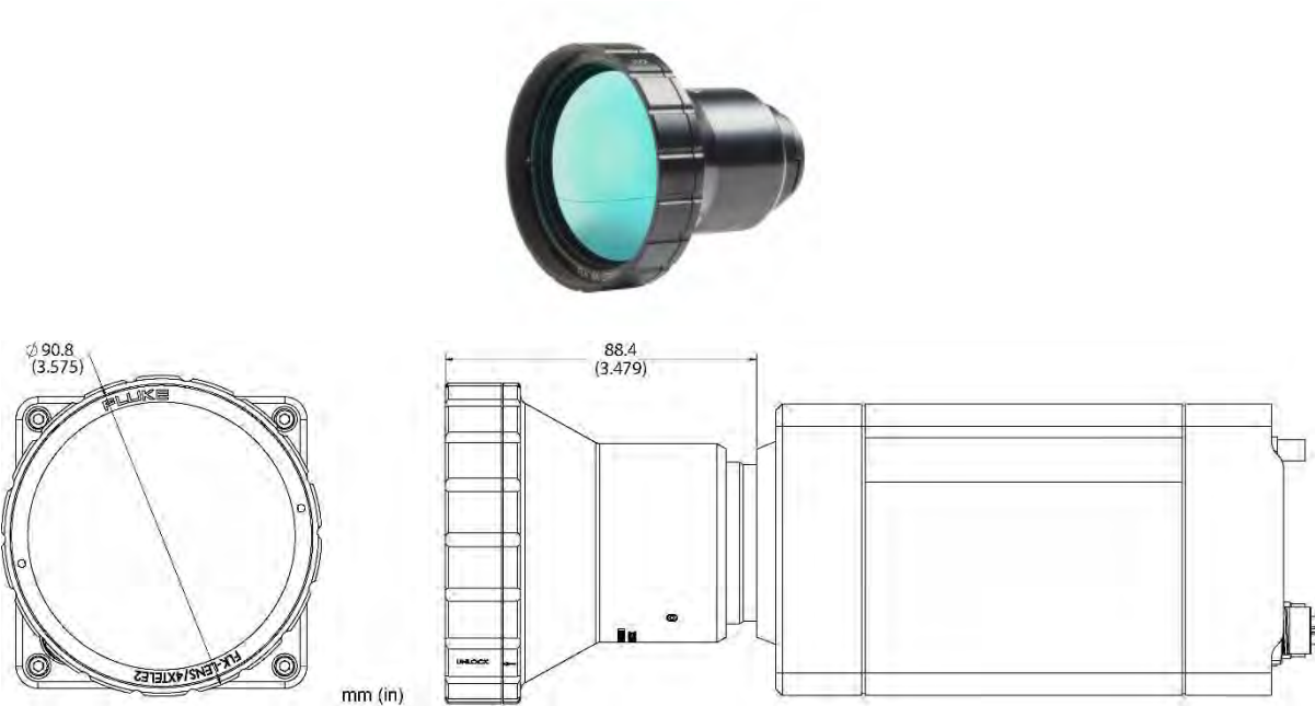
Figure 7-3: Tele Lens 4x
