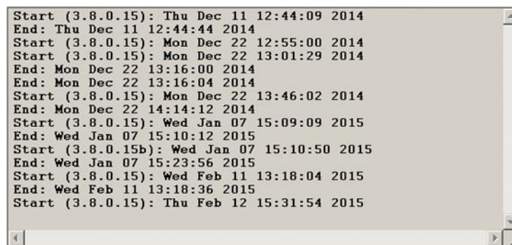
Figure 60: <Log-File> View
