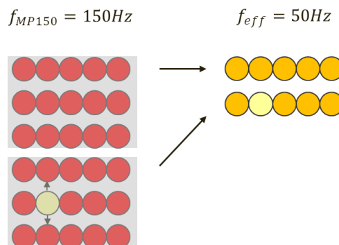
Figure 12: Data reduction with <Advanced Maximum> and a pixel with > 10 K difference to its neighbors
