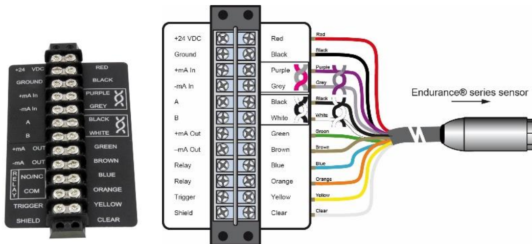
Figure 51: Terminal Block (E-TB) with wire color assignment
